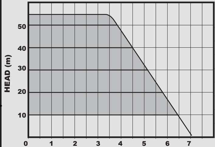
Performance Curves
