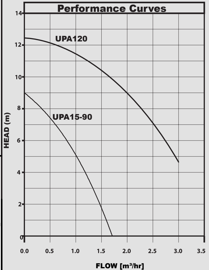
UPA BOOSTER 15_90
