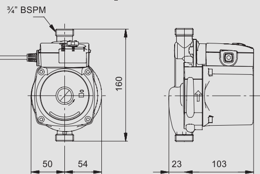
UPA BOOSTER 15_90
