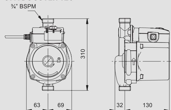
UPA BOOSTER 120
