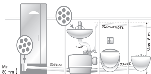
Sololift 2 WC-3 for toilet, sink and shower
