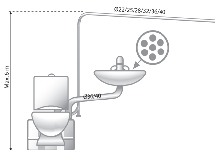
Sololift 2 WC-1 for single toilet
